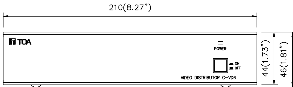
Front View
